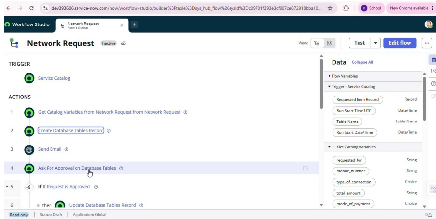
Fig 4: Network Request flow (FT-04)
